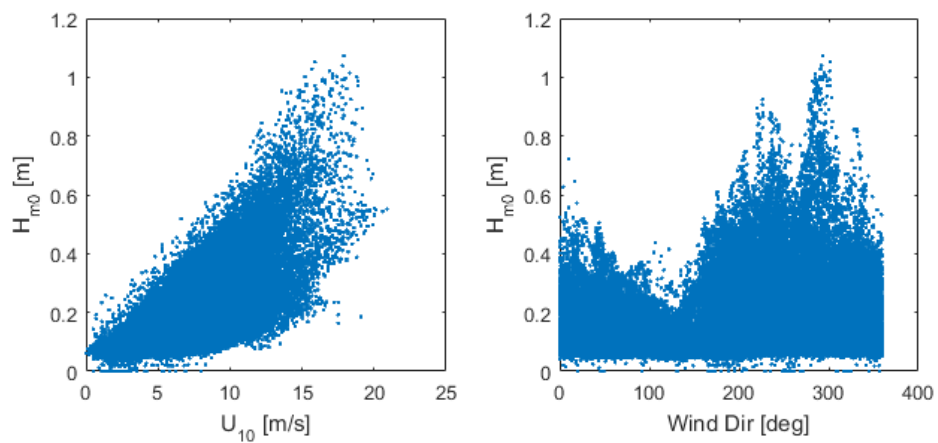
FIGURE 3.4: RELATIONSHIP BETWEEN WIND AND WAVE DATA COLLECTED AT MAROLLEGAT.
