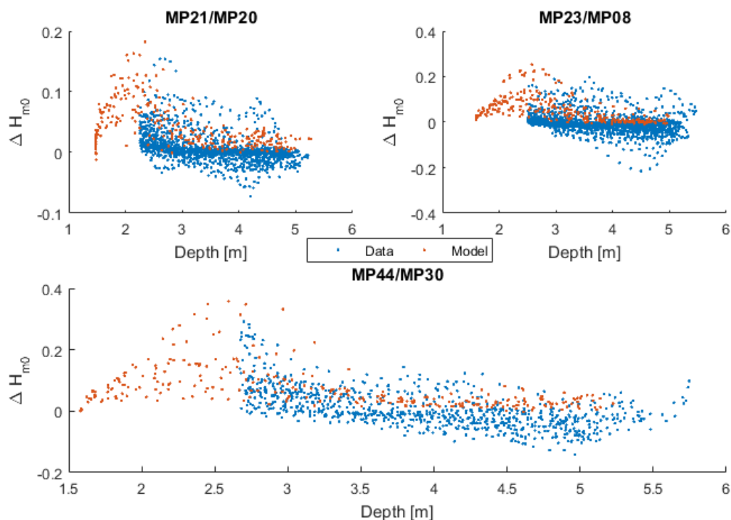
FIGURE 4.10: WAVE ATTENUATION/GROWTH OVER THE NOURISHMENT HOOK. POSITIVE VALUES INDICATE ATTENUATION, NEGATIVE VALUES INDICATE GROWTH.
