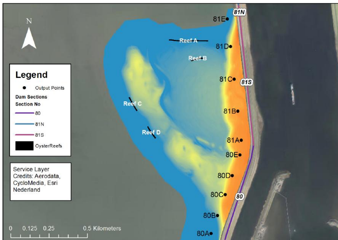
FIGURE 6.2: WAVE MODEL OUTPUT LOCATIONS AT THE DAM FOOT FOR INPUT INTO STRUCTURAL SAFETY CALCULATIONS. THE POINTS ARE LOCATED 30-50M FROM THE DAM FOOT.
