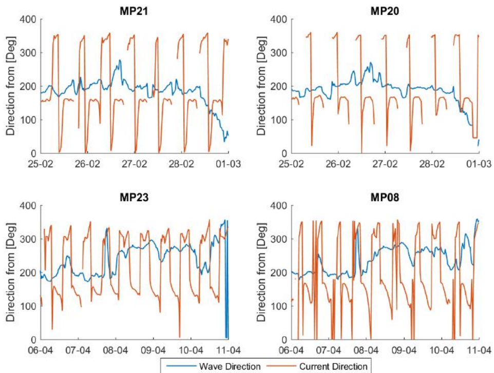
FIGURE 4.9: WAVE AND CURRENT DIRECTIONS DURING THE T1 PERIOD. BOTH CONVENTIONS ARE NAUTICAL.
