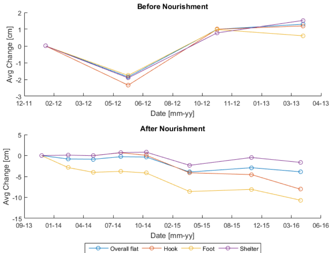
FIGURE 3.13: AVERAGE MEASURED BED LEVEL CHANGE AT THE OESTERDAM FLAT. THE HOOK, FOOT, AND SHELTER.
