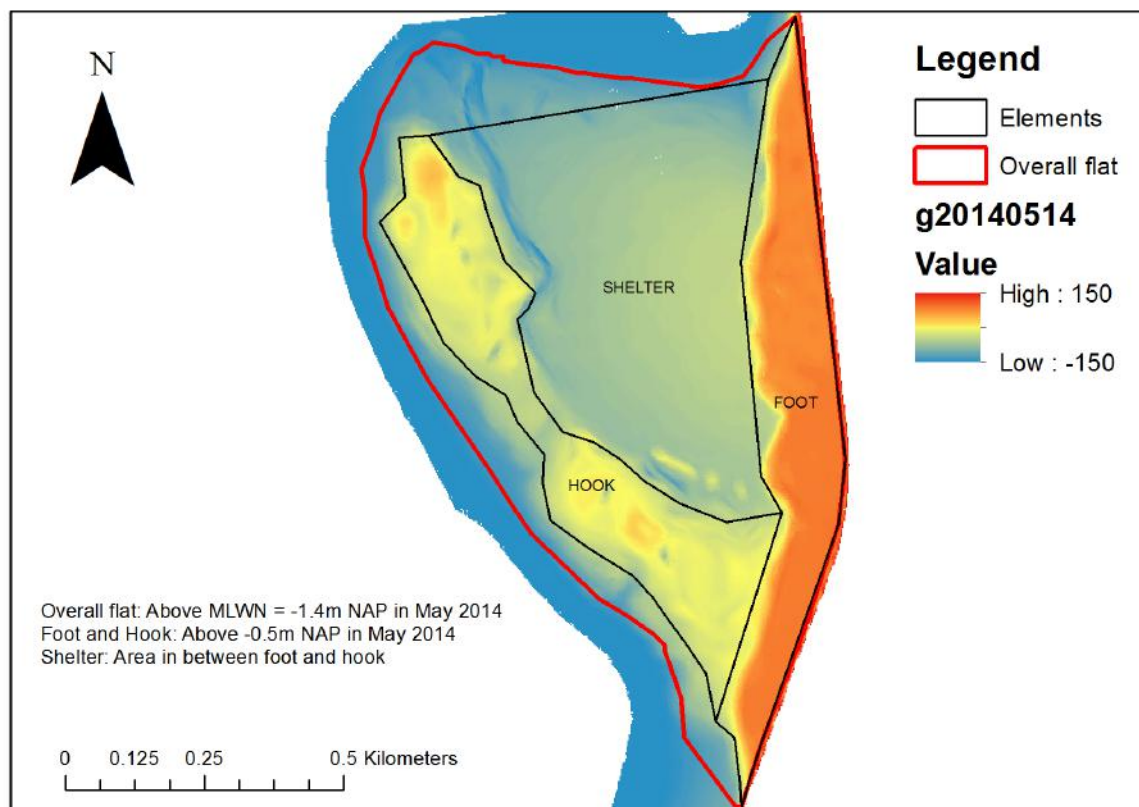
FIGURE 3.12: NOURISHMENT ELEMENTS DEFINED FOR TREND ANALYSIS OF EROSION FROM 2014 TO 2016.
