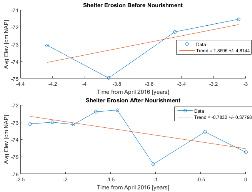
FIGURE A.20: TREND ANALYSIS OF EROSION IN THE SHELTERED AREA BETWEEN THE NOURISHMENT HOOK AND FOOT, BASED ON RTK SURVEYS.
