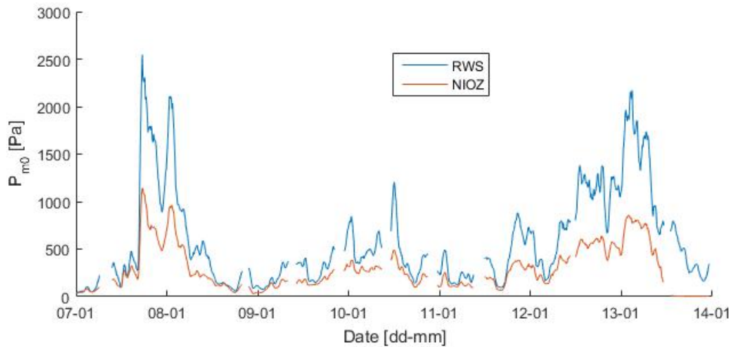
FIGURE 3.9: PROCESSING RESULTS FROM THE NIOZ AND RWS PRESSURE BOXES FOR THE T2 CAMPAIGN IN 2016.
