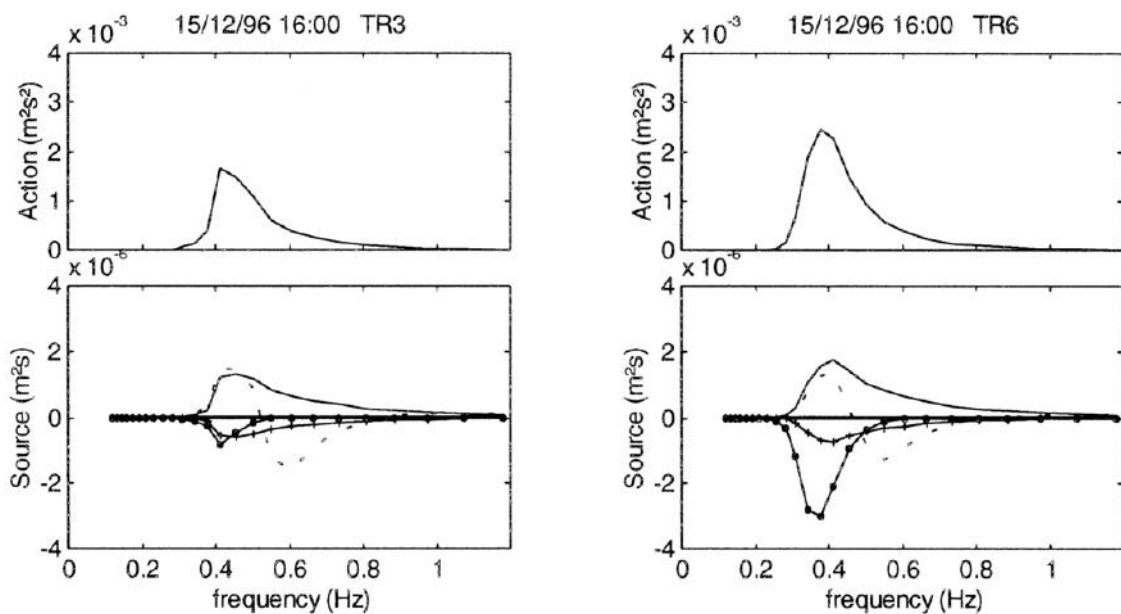
FIGURE 2.4: WAVE TRANSFORMATION IN MANUKAU HARBOR. SOURCE TERMS COMPUTED USING THE SWAN MODEL. (-) = WIND GROWTH, (+) = WHITECAPPING, (-) = QUADS, (-O-) = BOTTOM FRICTION. TAKEN FROM GORMAN & NEILSON (1999)
