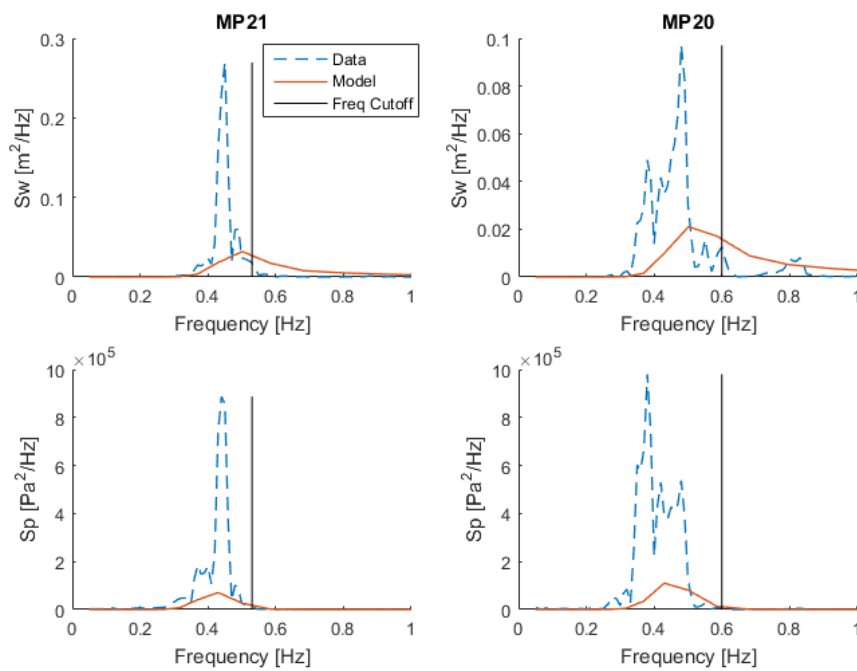
FIGURE 4.4: T1 OESTERDAM INITIAL WAVE SPECTRA (DEFAULT PARAMETERS) AT MP20 AND MP21 ON FEBRUARY 27 AT 2PM. THE BLACK LINES INDICATE THE FREQUENCY CUTOFF CORRESPONDING TO z/L = 0.5 .
