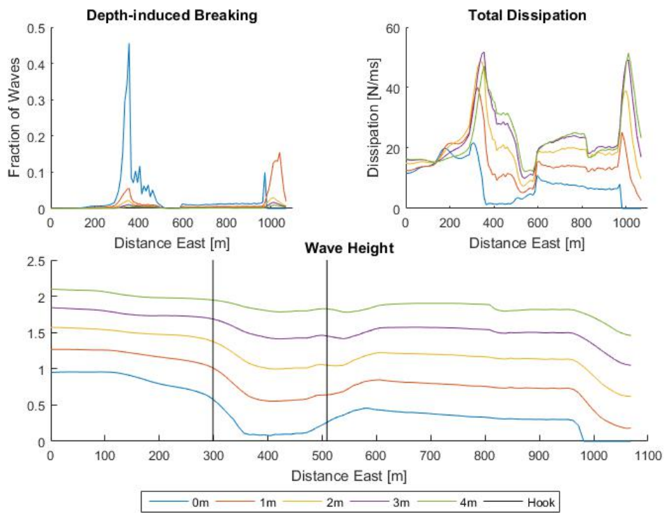
FIGURE 6.4: WAVE DISSIPATION AND GROWTH OVER THE OESTERDAM FLAT FOR THE REAL NOURISHMENT SCENARIO. 2020 FAST EROSION TIME POINT.
