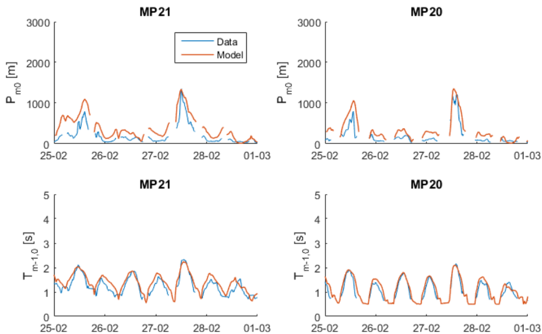
FIGURE 4.6: T1 OESTERDAM SIMULATIONS WITH CALIBRATED WAVE PERIODS USING SCALED UP QUADRUPLLET INTERACTIONS.
