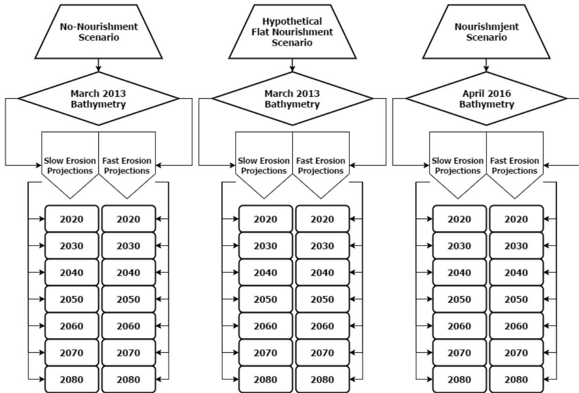
FIGURE 6.1: SCENARIOS FOR SIMULATION OF DESIGN CONDITIONS AT THE OESTERDAM.
