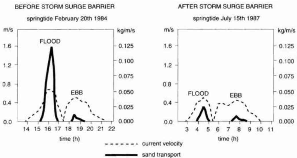
FIGURE 2.9: CHANGES IN SEDIMENT IMPORT DURING FLOOD TIDE AND EXPORT DURING EBB TIDE BEFORE AND AFTER THE CONSTRUCTION OF THE STORM SURGE BARRIER. TAKEN FROM LOUTERS ET AL. (1998) ; PEZIJ (2015) .
