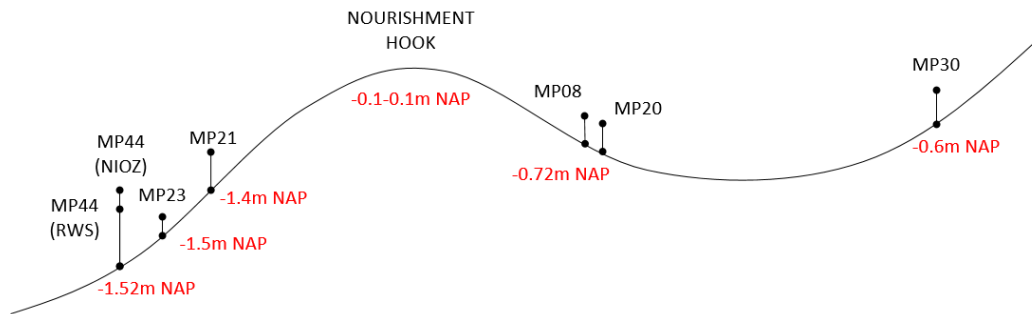
FIGURE 3.7: SCHEMATIZED CROSS SECTION OF NOURISHMENT HOOK (NOT TO SCALE).
