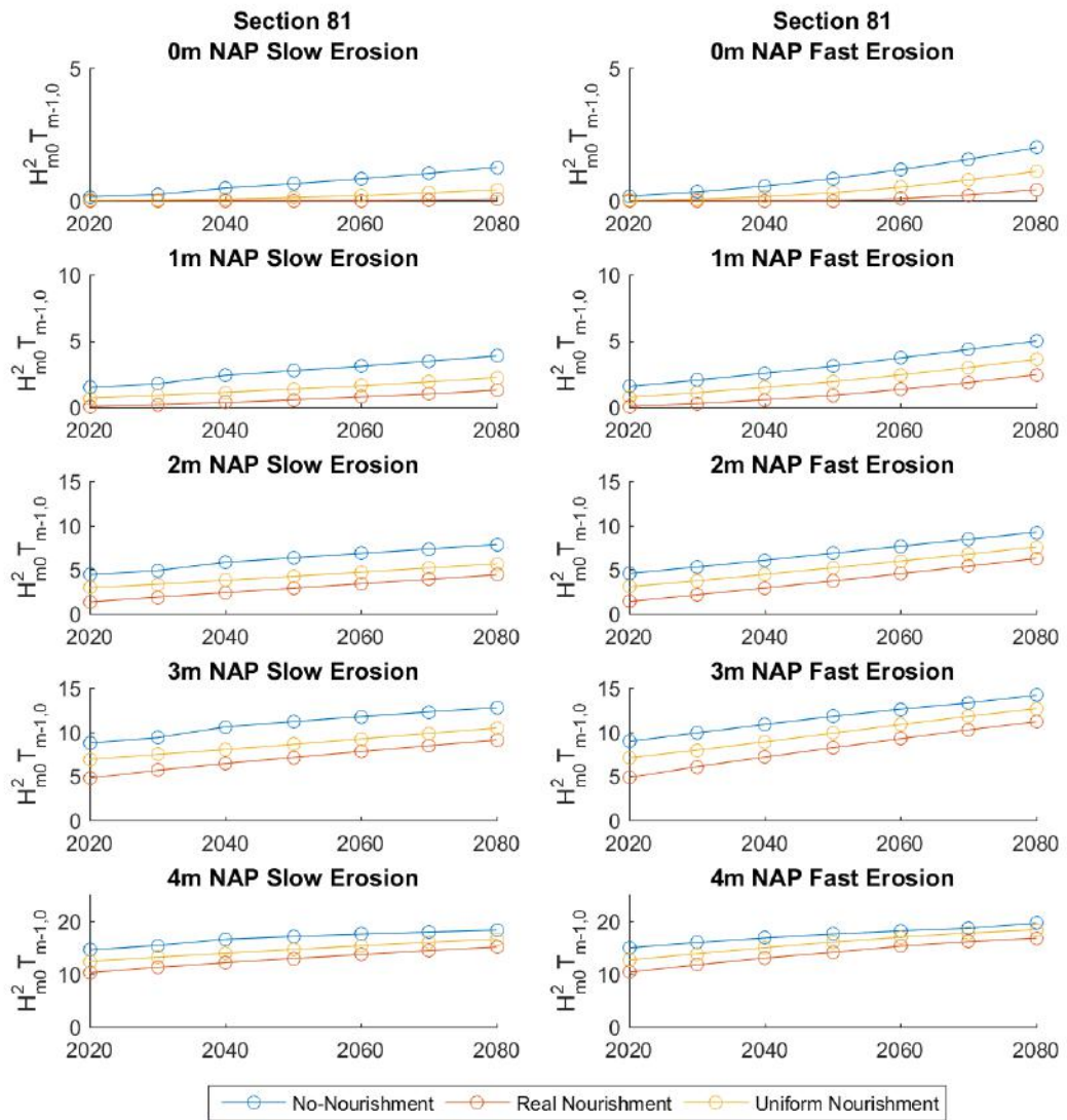
FIGURE 6.3: LOAD FUNCTION Z1=H_s*H_s*T_m . PROJECTED TO 2080 IN THE SLOW AND FAST EROSION PROJECTION SCENARIOS. SECTION 81S OF THE OESTERDAM.
