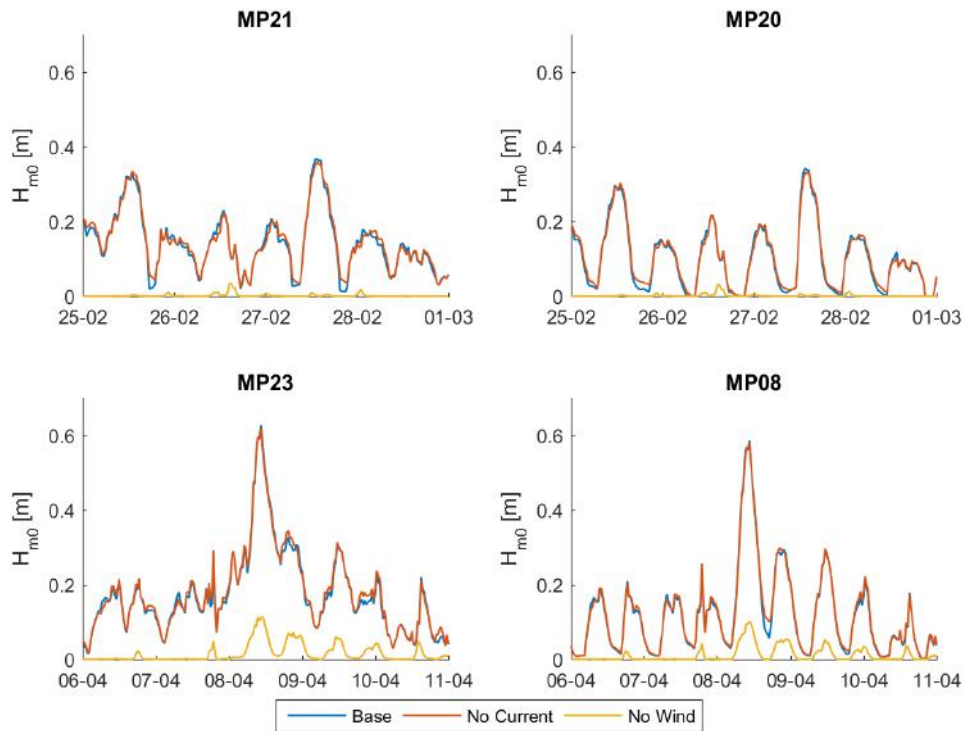
FIGURE 4.8: SENSITIVITY OF WAVE HEIGHT TO SIMULATED CURRENTS AND WIND FORCING.
