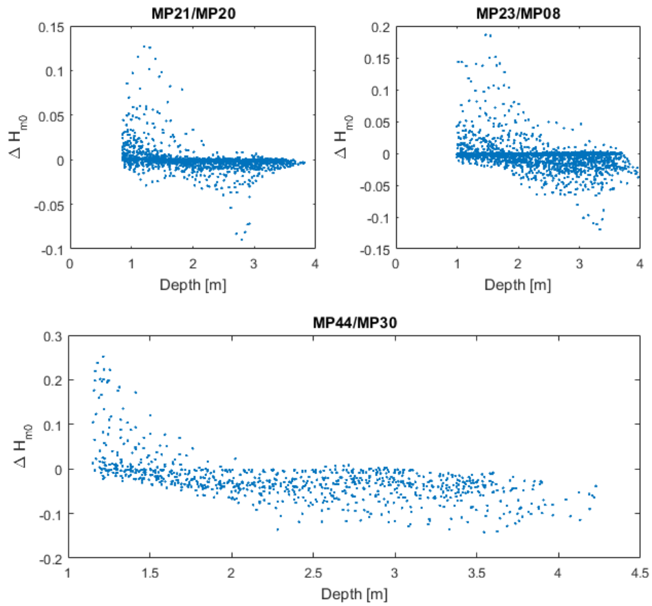
FIGURE 3.8: WAVE ATTENUATION/GROWTH OVER THE NOURISHMENT HOOK. POSITIVE VALUES INDICATE ATTENUATION, NEGATIVE VALUES INDICATE GROWTH.
