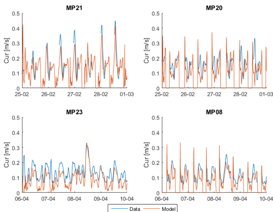
FIGURE 4.7: T1 OESTERDAM MODELLED CURRENTS.
