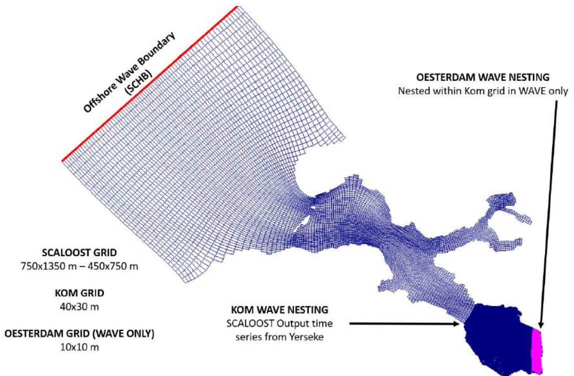
FIGURE 4.2: DELFT3D WAVE GRIDS FOR SCALOOST, THE KOM, AND THE OESTERDAM.
