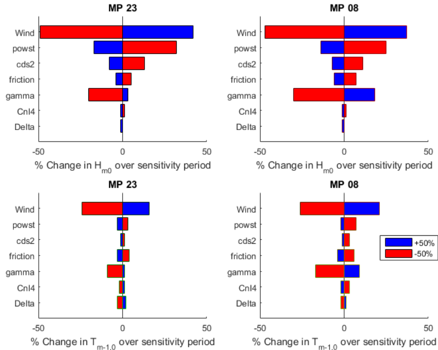
FIGURE 4.5: TORNADO DIAGRAMS OF SWAN PARAMETERS SHOWING THE SENSITIVITY OF WAVE HEIGHT AND PERIOD AT THE NOURISHMENT LOCATION.
