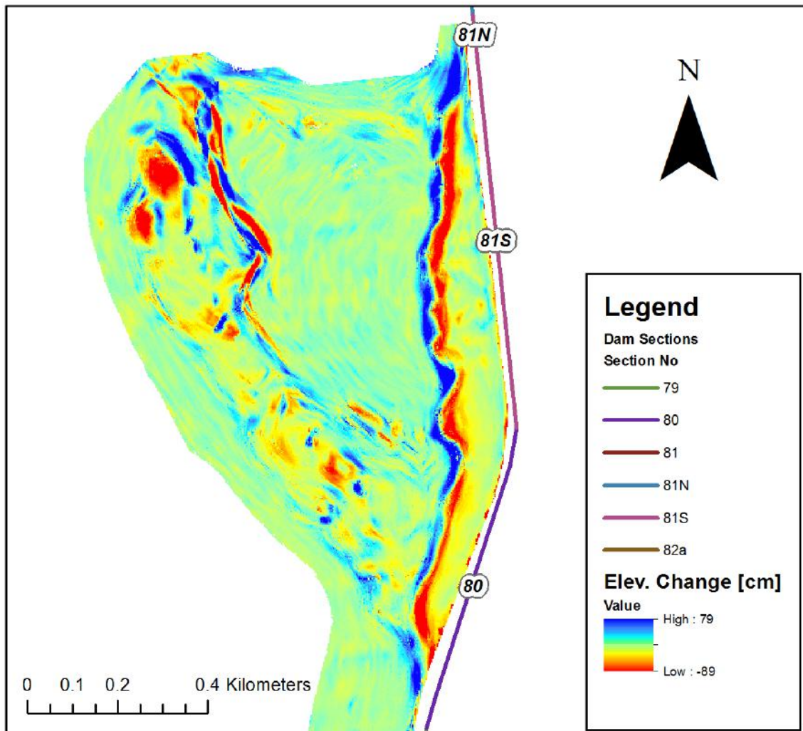
FIGURE 3.11: EROSION AND SPREADING OF THE NOURISHMENT FROM MAY 14, 2014 TO OCTOBER 29, 2015. BLUE INDICATES ACCRETION, RED INDICATES EROSION.
