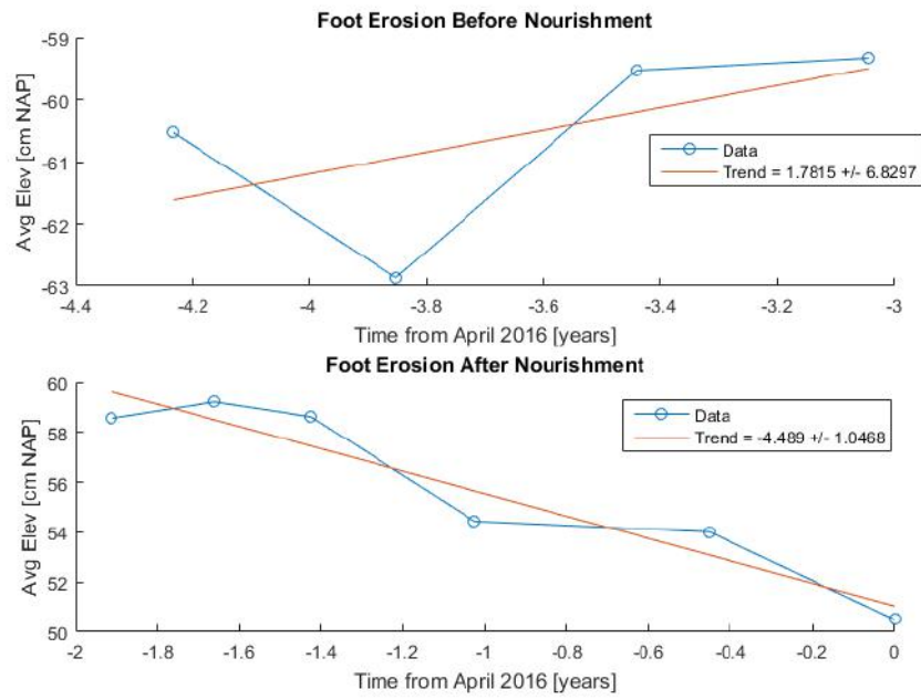
FIGURE A.18: TREND ANALYSIS OF THE NOURISHMENT FOOT EROSION BASED ON RTK SURVEYS.
