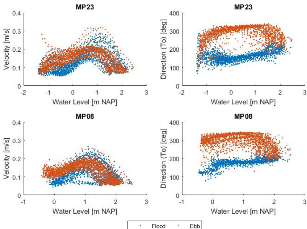
FIGURE 3.10: FLOOD AND EBB TIDAL CURRENTS AT THE MP23 AND MP08 LOCATIONS. DIRECTIONS ARE TOWARDS, OPPOSITE TO THE WIND/WAVE CONVENTION.
