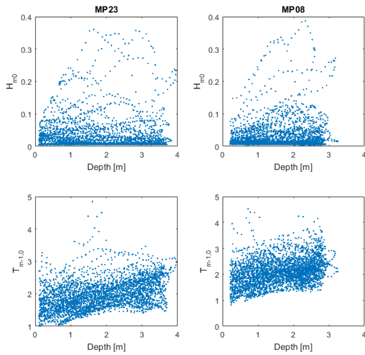
FIGURE A.8: WATER DEPTH AND WAVES AT MP23 AND MP08.
