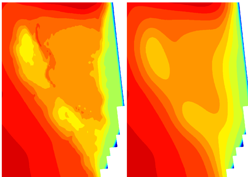
FIGURE 5.2: ESTIMATED NOURISHMENT SPREADING FROM 2020 TO 2080 IN DELFT3D USING A SMOOTHING FUNCTION IN QUICKIN.
