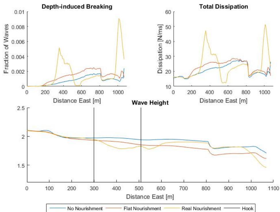
FIGURE 6.5: WAVE DISSIPATION AND GROWTH OVER THE OESTERDAM FLAT DURING DESIGN CONDITIONS AT THE 4M WATER LEVEL. 2020 FAST EROSION TIME POINT.
