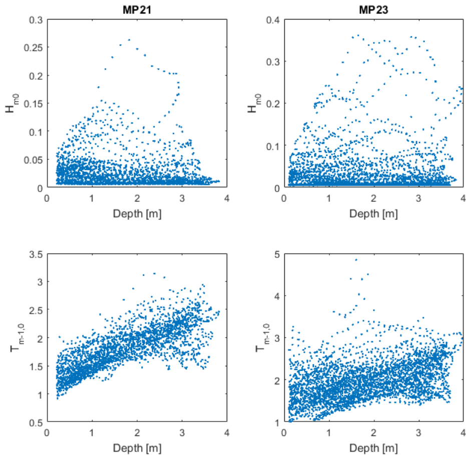
FIGURE 3.6: TIDAL MODULATION OF WAVES AT NOURISHMENT.
