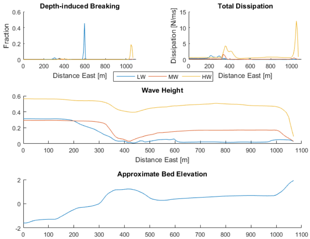
FIGURE 4.11: MODELLED WAVE ATTENUATION ALONG NORTHERN TRANSECT DURING HIGH WATER, MEAN WATER, AND LOW WATER IN APRIL 2014.
