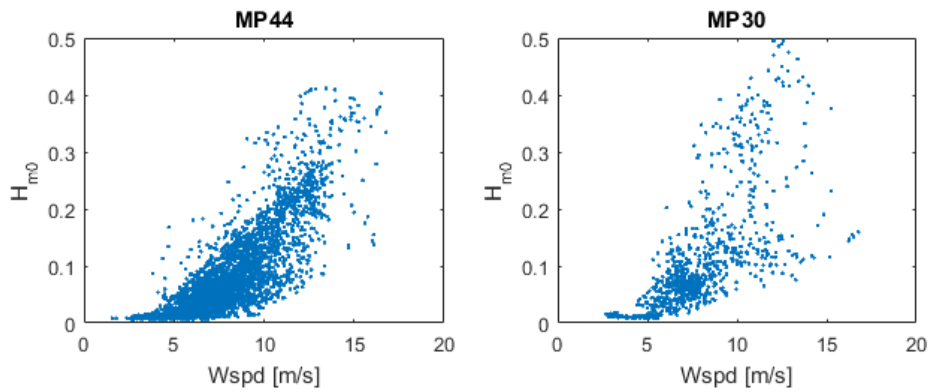
FIGURE 3.5: RELATIONSHIP BETWEEN MRG WIND AND PRESSURE BOX WAVE HEIGHTS.
