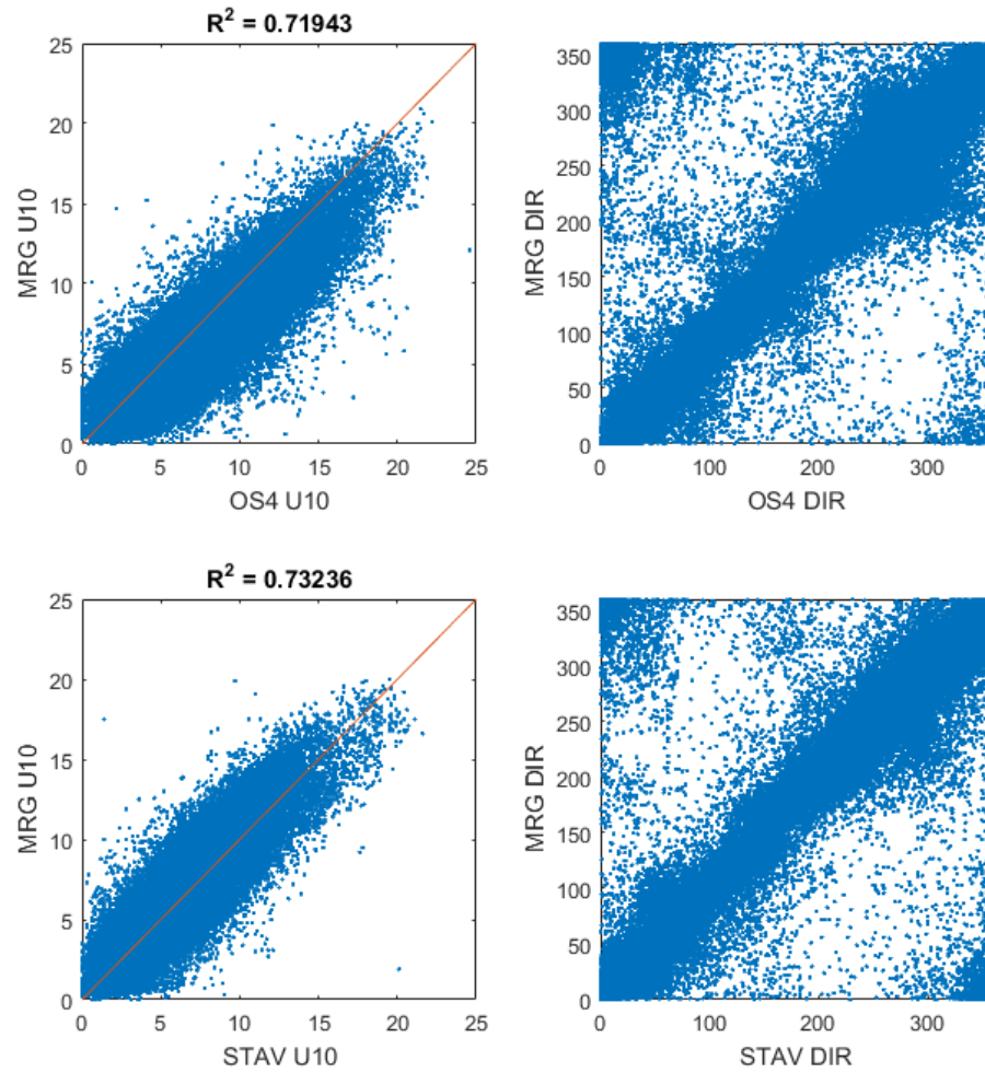
FIGURE 3.3: MAROLLEGAT WINDS CORRELATED WITH STAVENISSE AND OOSTERSCHELDE 4.
