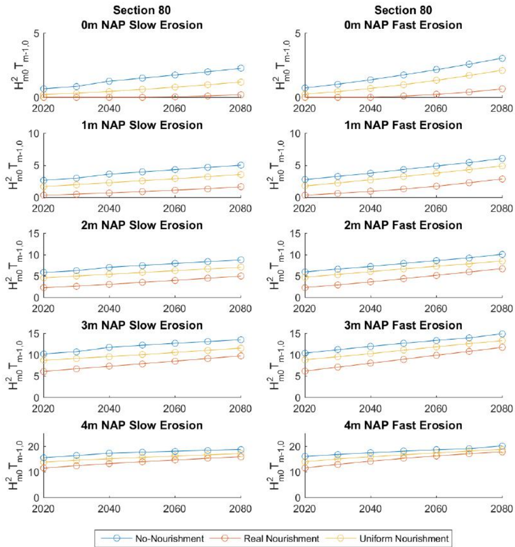
FIGURE C.7: LOAD FUNCTION Z_3=H_s*H_s*T_m . PROJECTED TO 2080 IN THE SLOW AND FAST EROSION PROJECTION SCENARIOS. SECTION 80 OF THE OESTERDAM.
