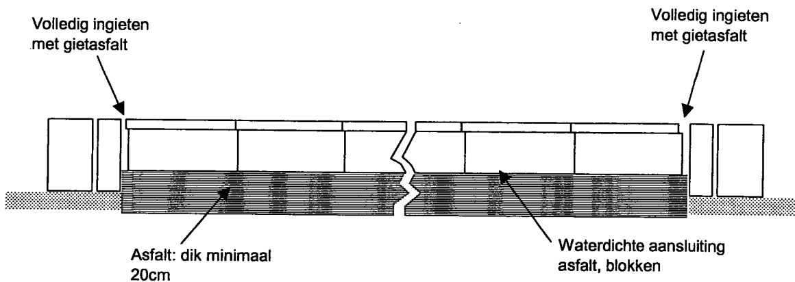
Langsdoorsnede museumglooiing
